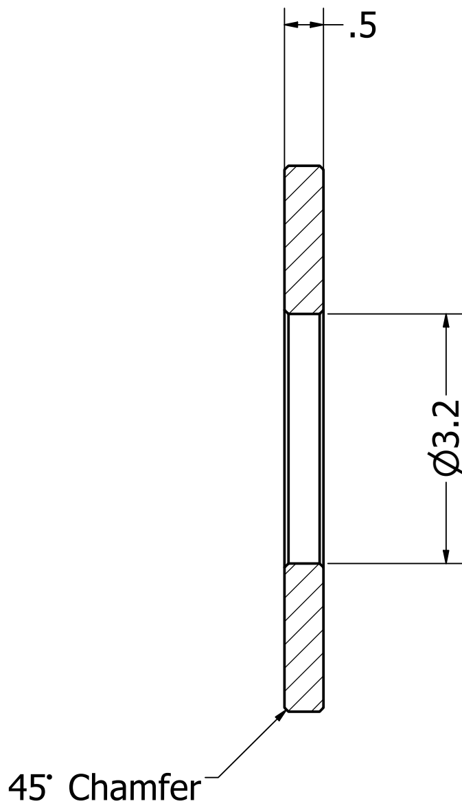
SECTION A-A SCALE 15: 1
